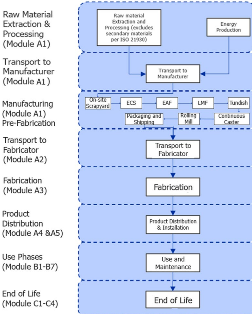
Figure 1: Flow chart for product system
